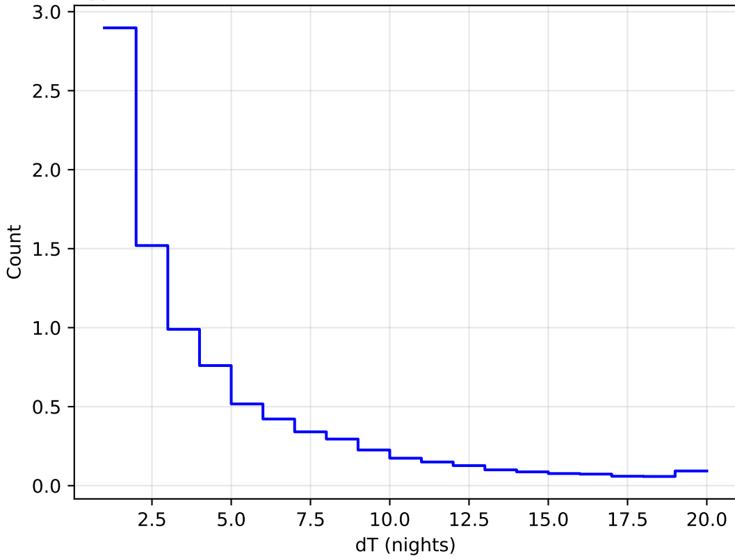
too_5_1v3.4_10yrs All sky all bands: DeltaNight Histogram 1e6
