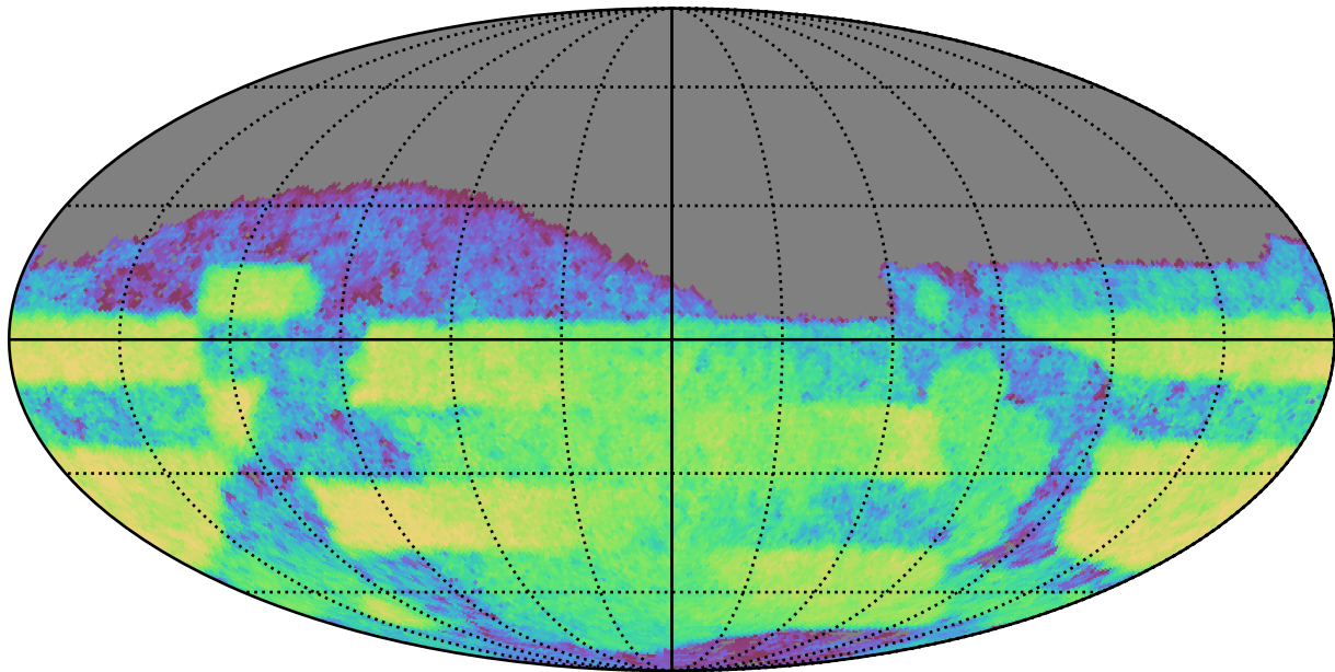
too_5_1v3.4_10yrs Yr 3-4 z band: CoaddM5
