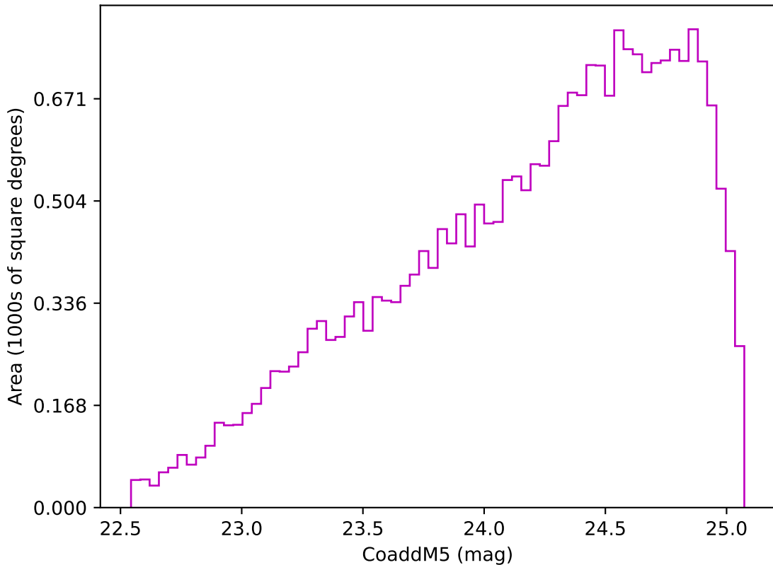
too_5_1v3.4_10yrs Yr 3-4 z band: CoaddM5
