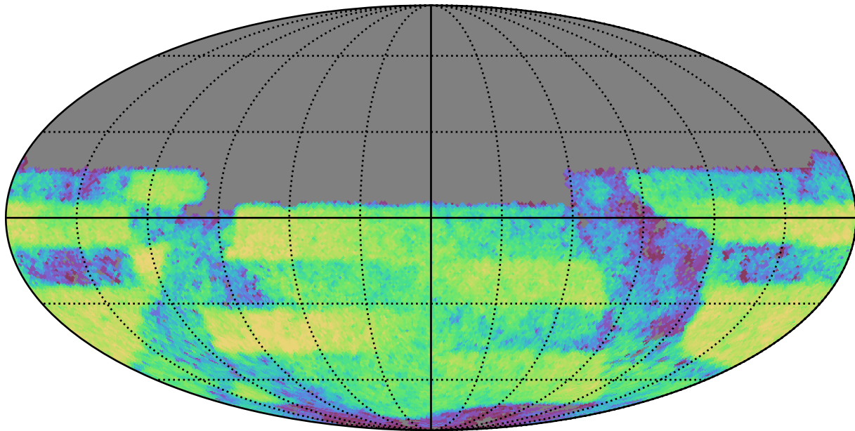
too_5_1v3.4_10yrs Yr 3-4 y band: CoaddM5
