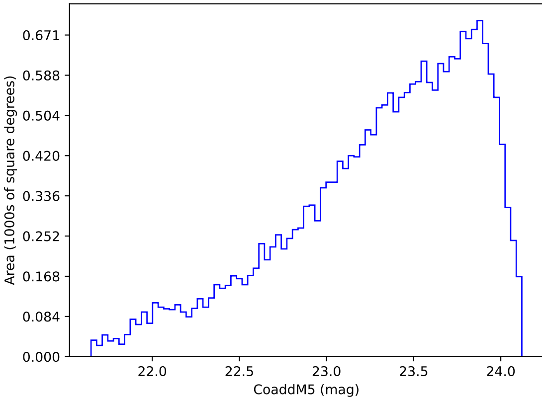
too_5_1v3.4_10yrs Yr 3-4 y band: CoaddM5
