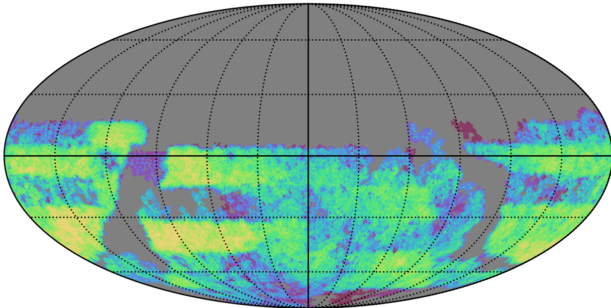
too_5_1v3.4_10yrs Yr 3-4 u band: CoaddM5
