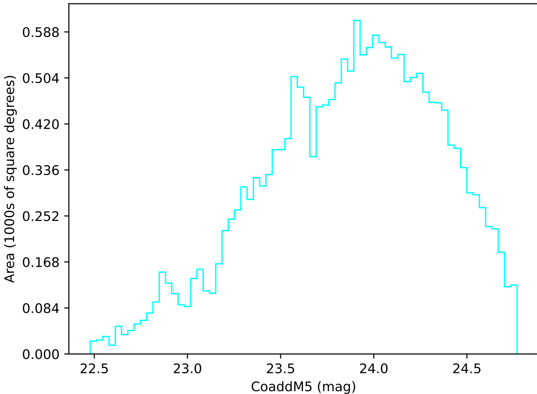
too_5_1v3.4_10yrs Yr 3-4 u band: CoaddM5
