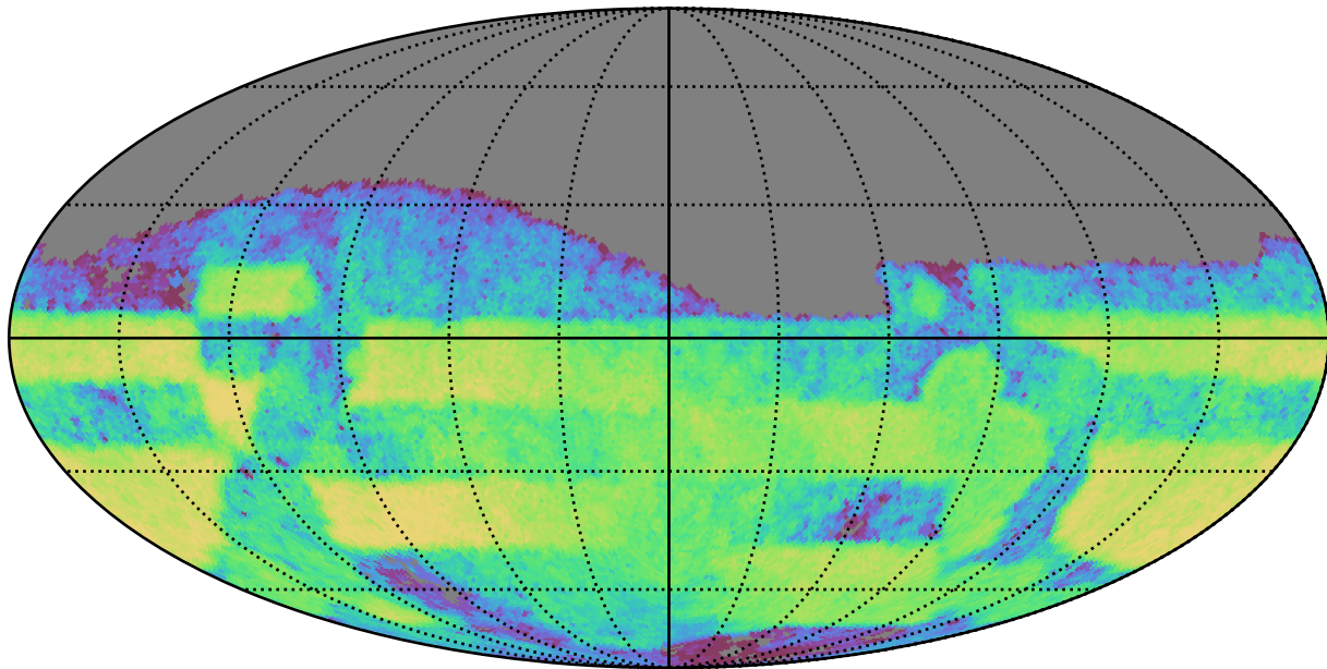
too_5_1v3.4_10yrs Yr 3-4 i band: CoaddM5
