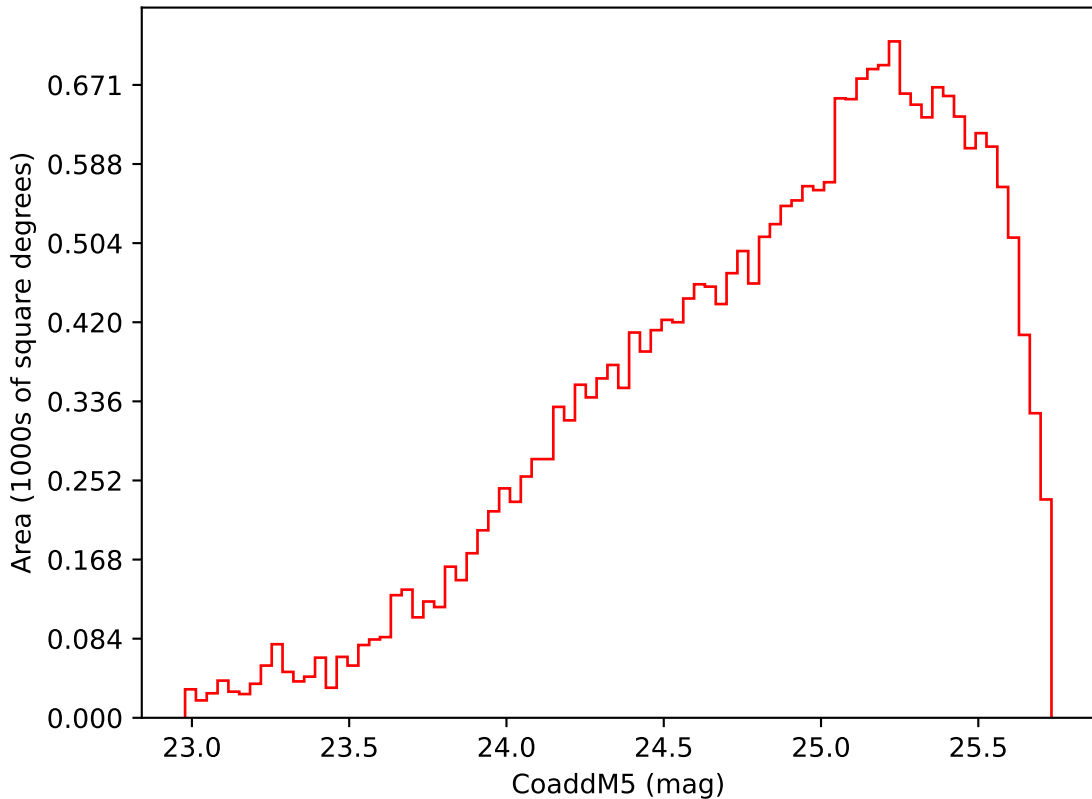
too_5_1v3.4_10yrs Yr 3-4 i band: CoaddM5
