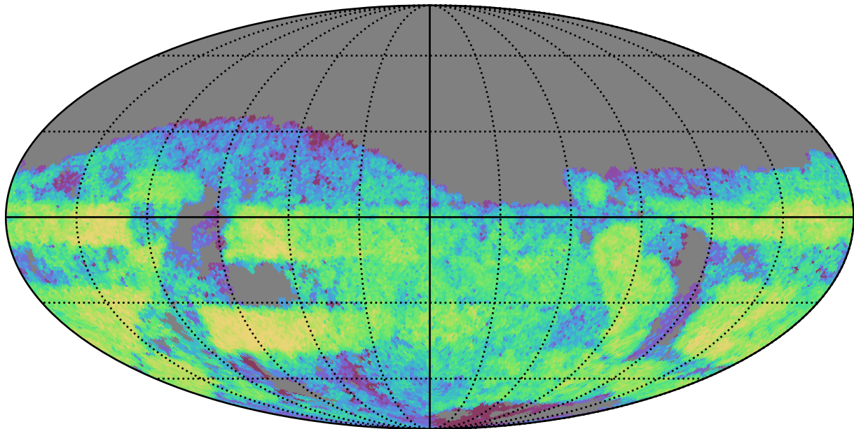
too_5_1v3.4_10yrs Yr 3-4 g band: CoaddM5
