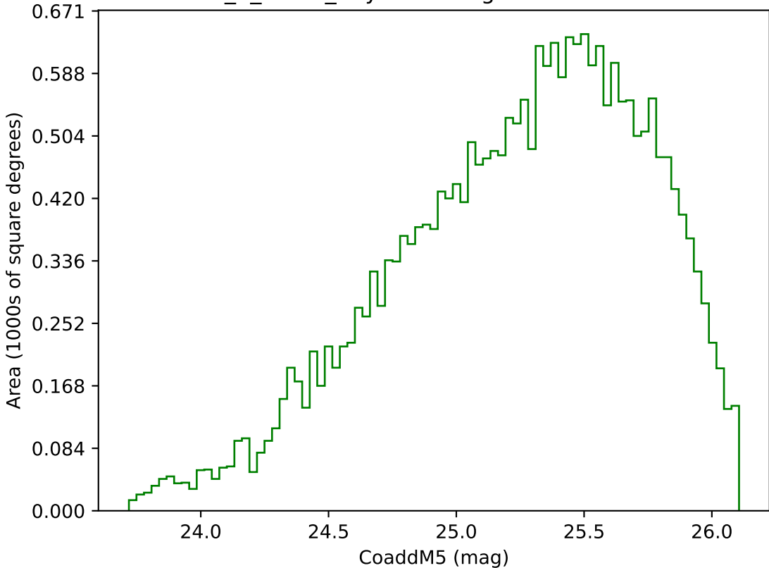
too_5_1v3.4_10yrs Yr 3-4 g band: CoaddM5
