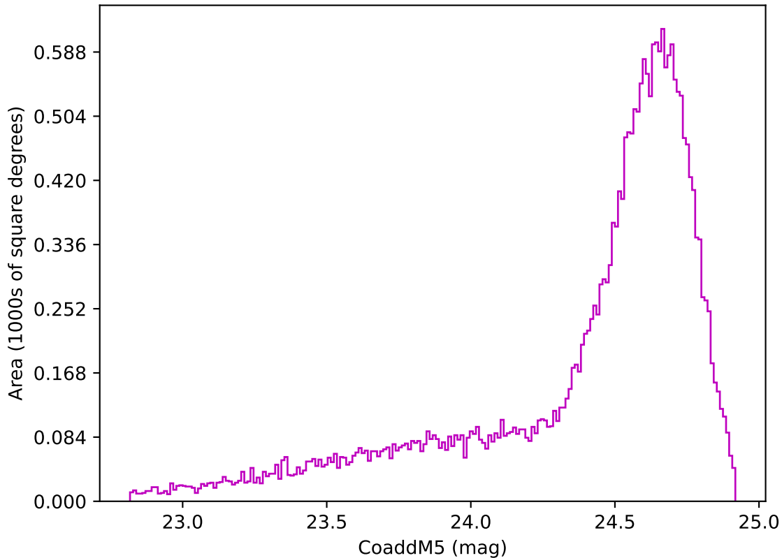
too_5_1v3.4_10yrs Yr 1 z band: CoaddM5
