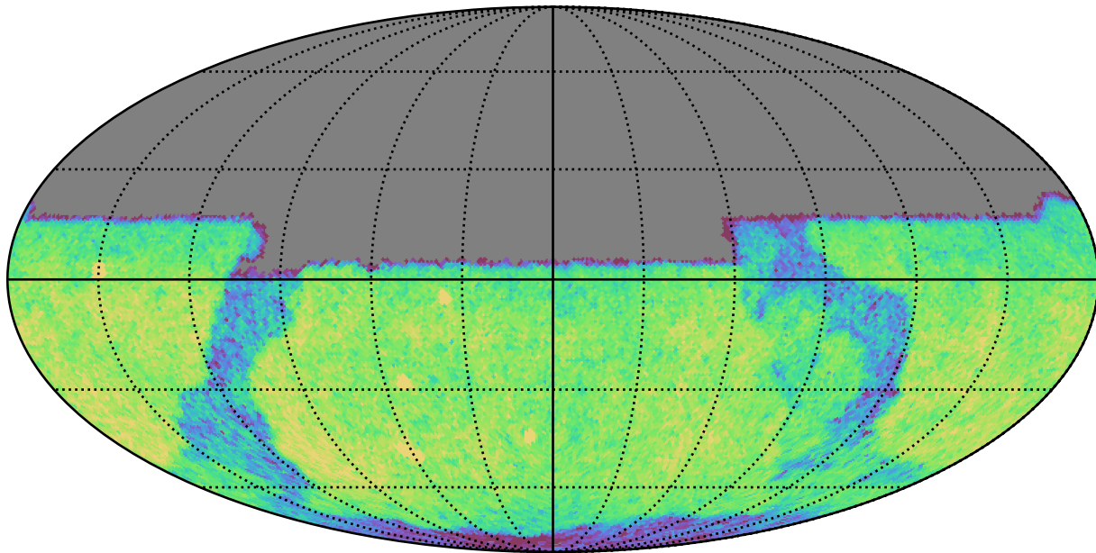
too_5_1v3.4_10yrs Yr 1 y band: CoaddM5
