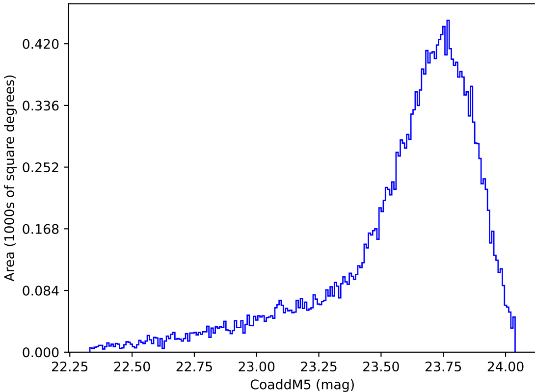
too_5_1v3.4_10yrs Yr 1 y band: CoaddM5
