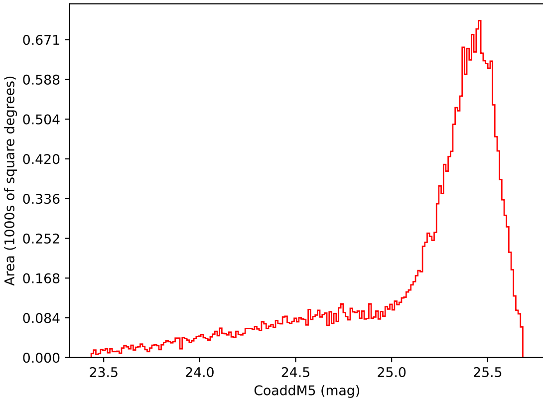
too_5_1v3.4_10yrs Yr 1 i band: CoaddM5
