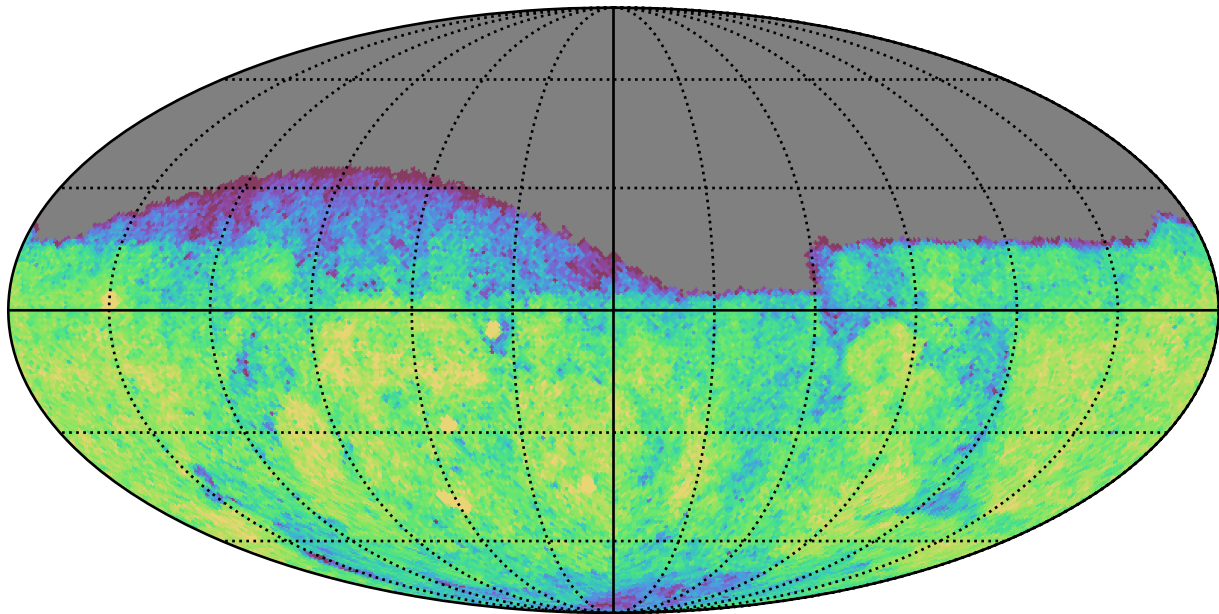
too_5_1v3.4_10yrs Yr 1 g band: CoaddM5
