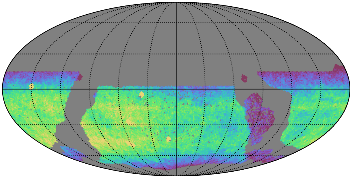
too_5_1v3.4_10yrs WFD y band: CoaddM5
