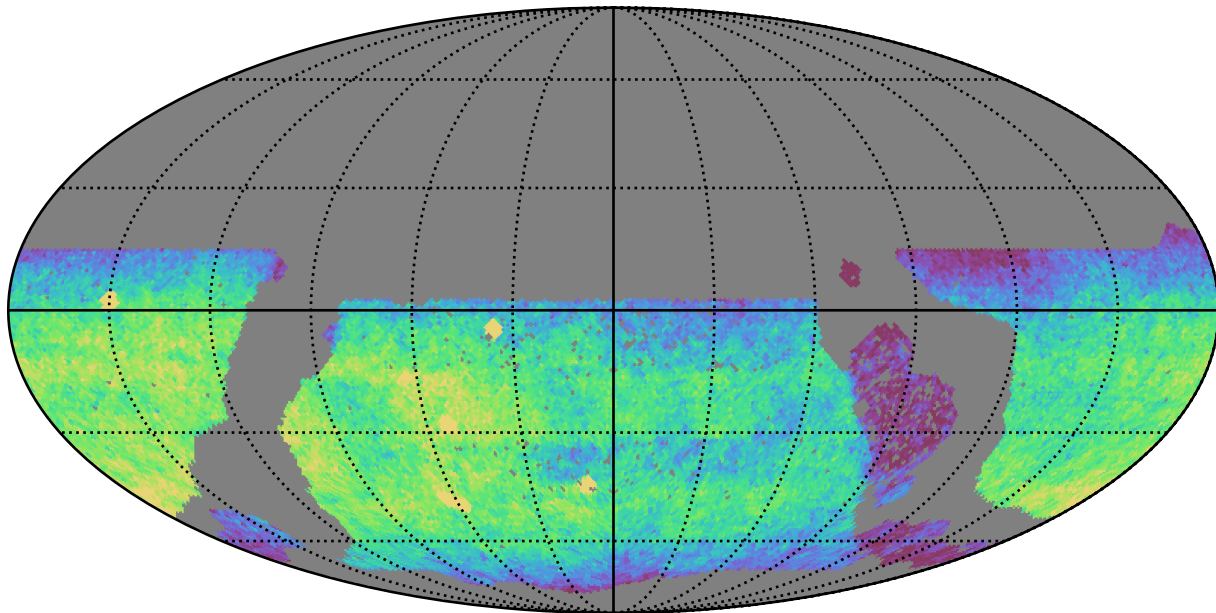
too_5_1v3.4_10yrs WFD u band: CoaddM5
