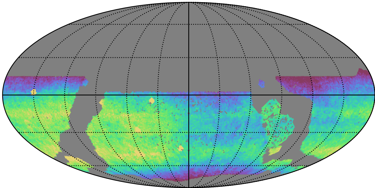
too_5_1v3.4_10yrs WFD r band: CoaddM5
