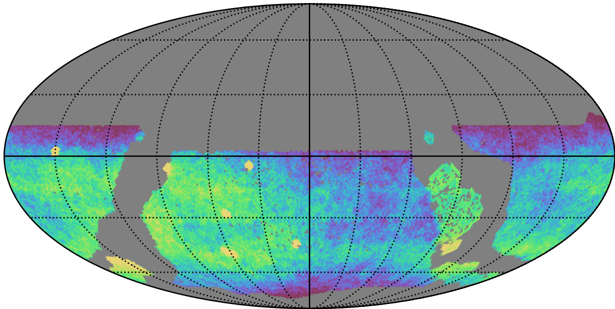
too_5_1v3.4_10yrs WFD g band: CoaddM5
