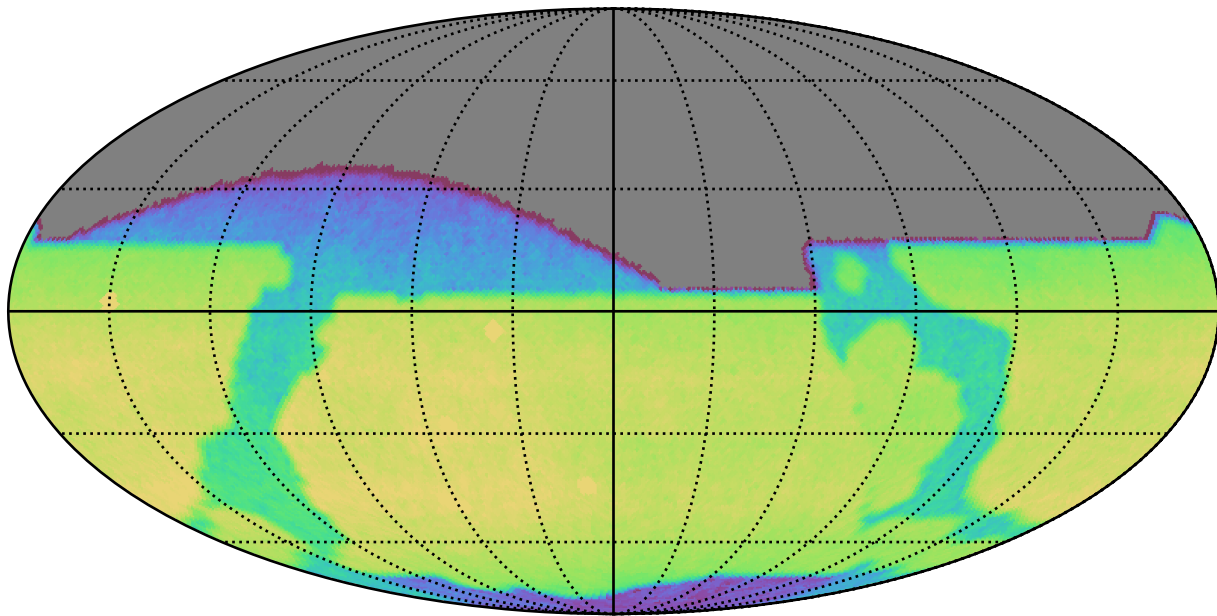
too_5_1v3.4_10yrs All sky z band: CoaddM5
