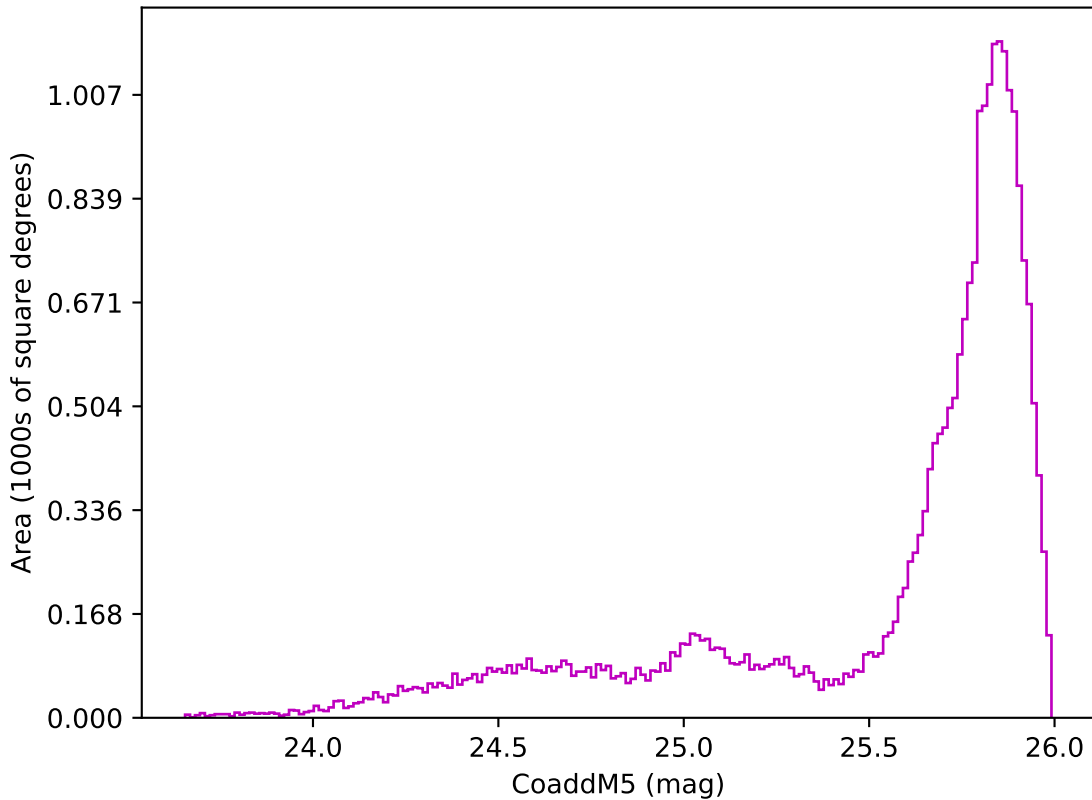
too_5_1v3.4_10yrs All sky z band: CoaddM5
