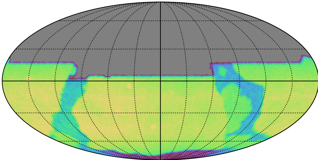
too_5_1v3.4_10yrs All sky y band: CoaddM5
