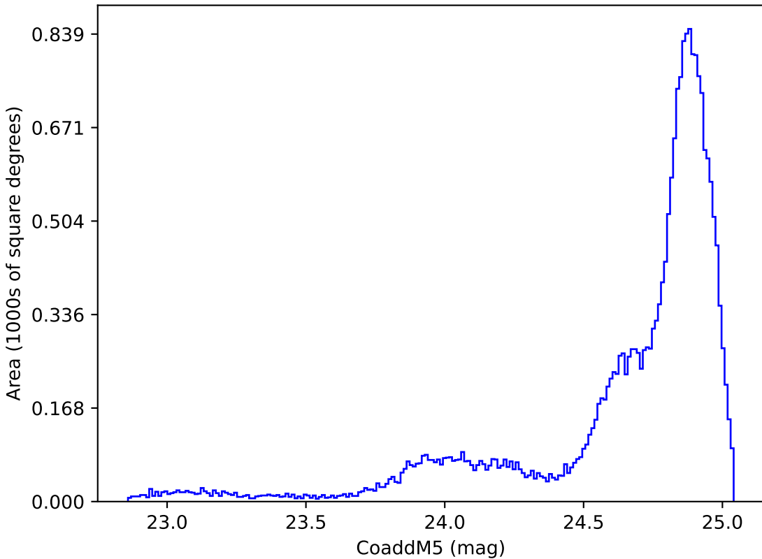
too_5_1v3.4_10yrs All sky y band: CoaddM5
