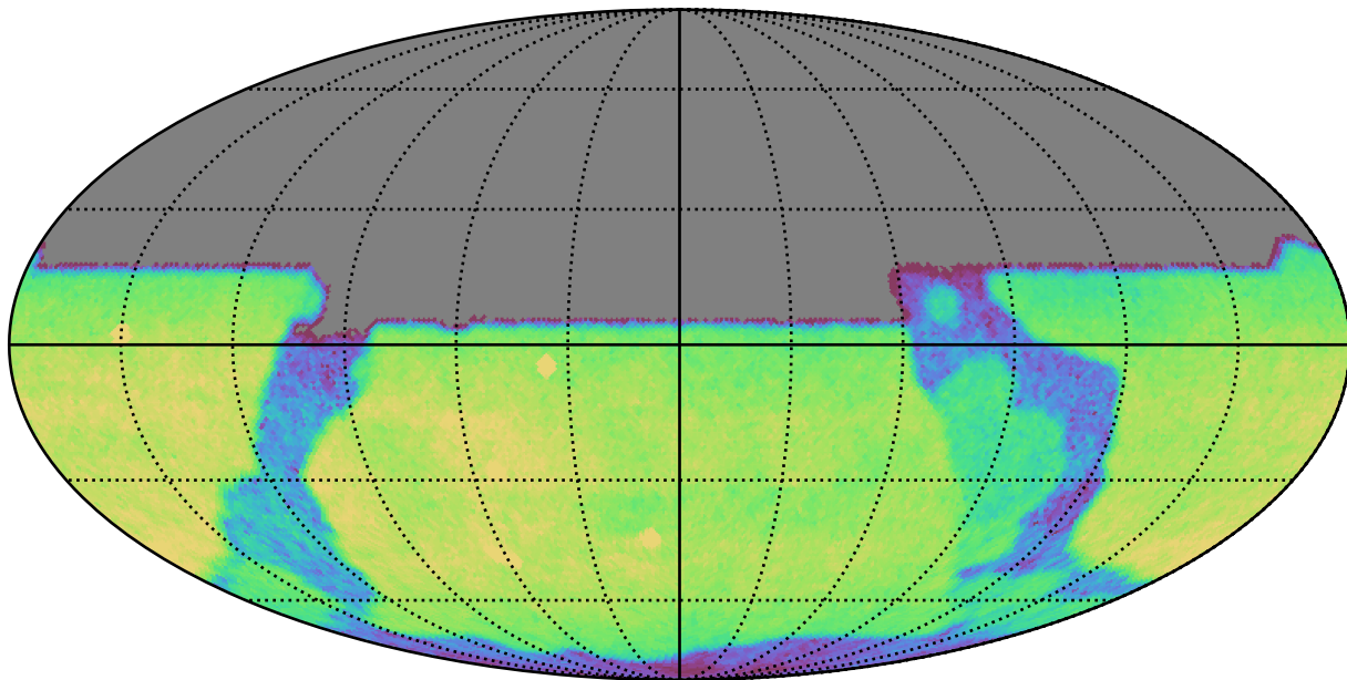
too_5_1v3.4_10yrs All sky u band: CoaddM5
