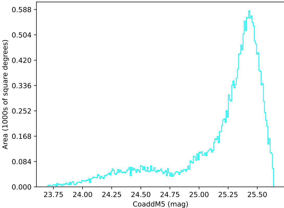
too_5_1v3.4_10yrs All sky u band: CoaddM5
