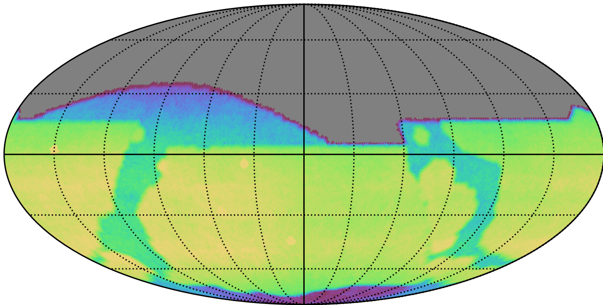
too_5_1v3.4_10yrs All sky r band: CoaddM5
