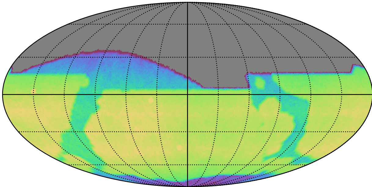
too_5_1v3.4_10yrs All sky i band: CoaddM5
