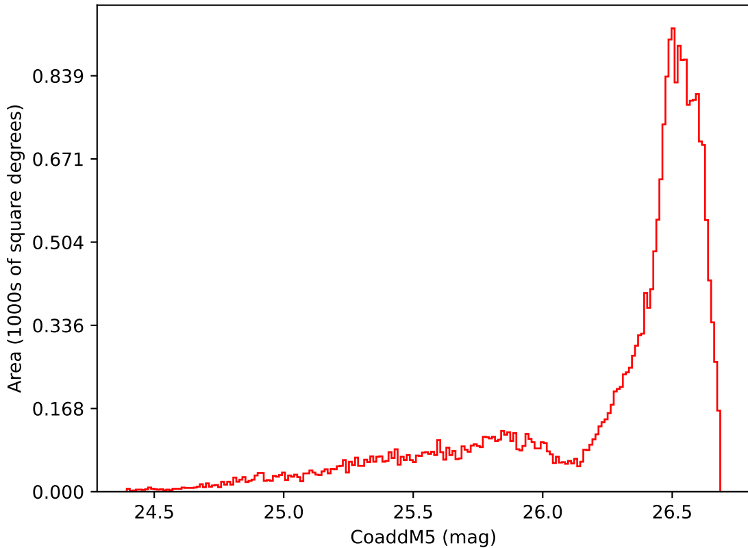
too_5_1v3.4_10yrs All sky i band: CoaddM5
