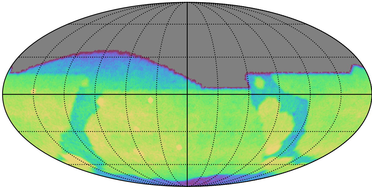
too_5_1v3.4_10yrs All sky g band: CoaddM5
