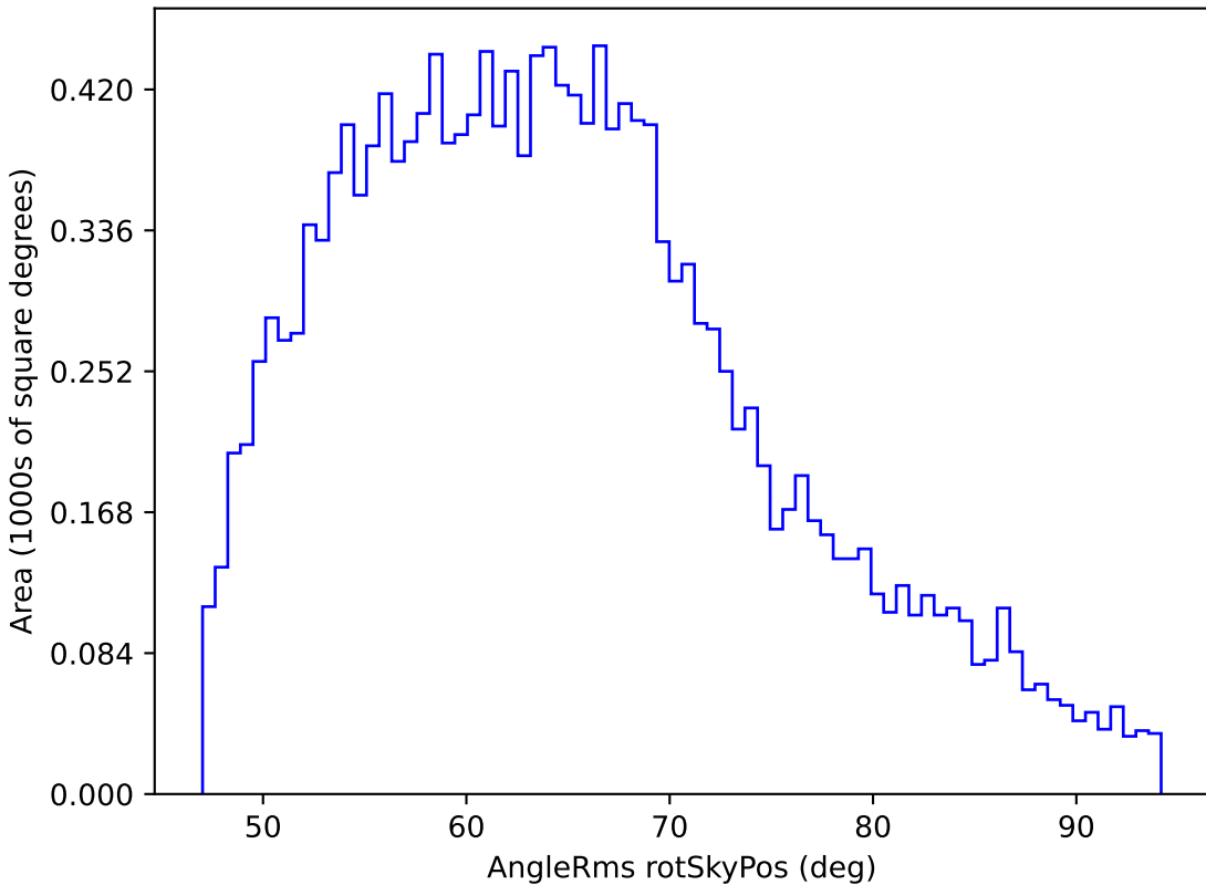
too_5_1v3.4_10yrs WFD z band: AngleRms rotSkyPos
