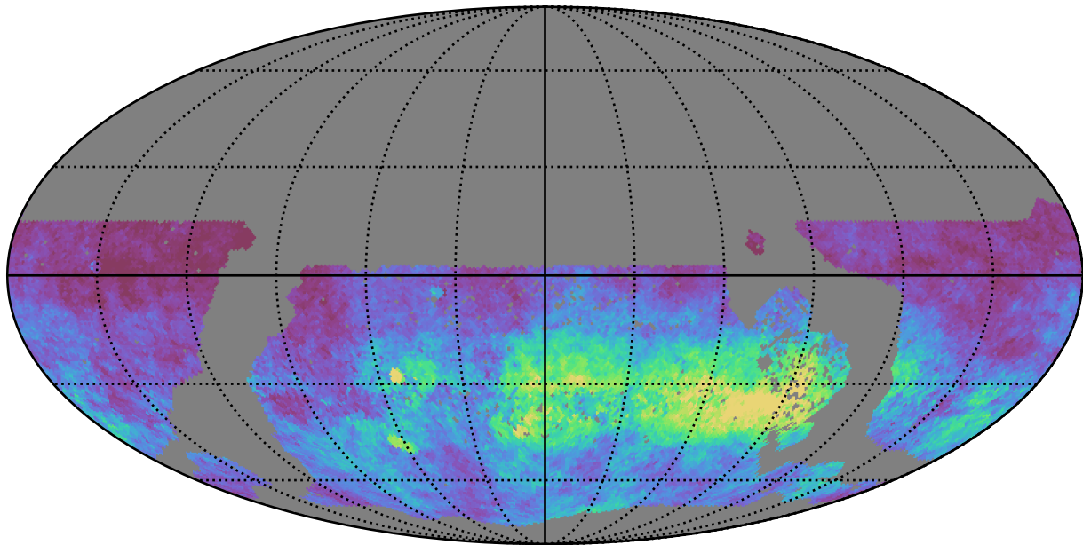
too_5_1v3.4_10yrs WFD y band: AngleRms rotSkyPos
