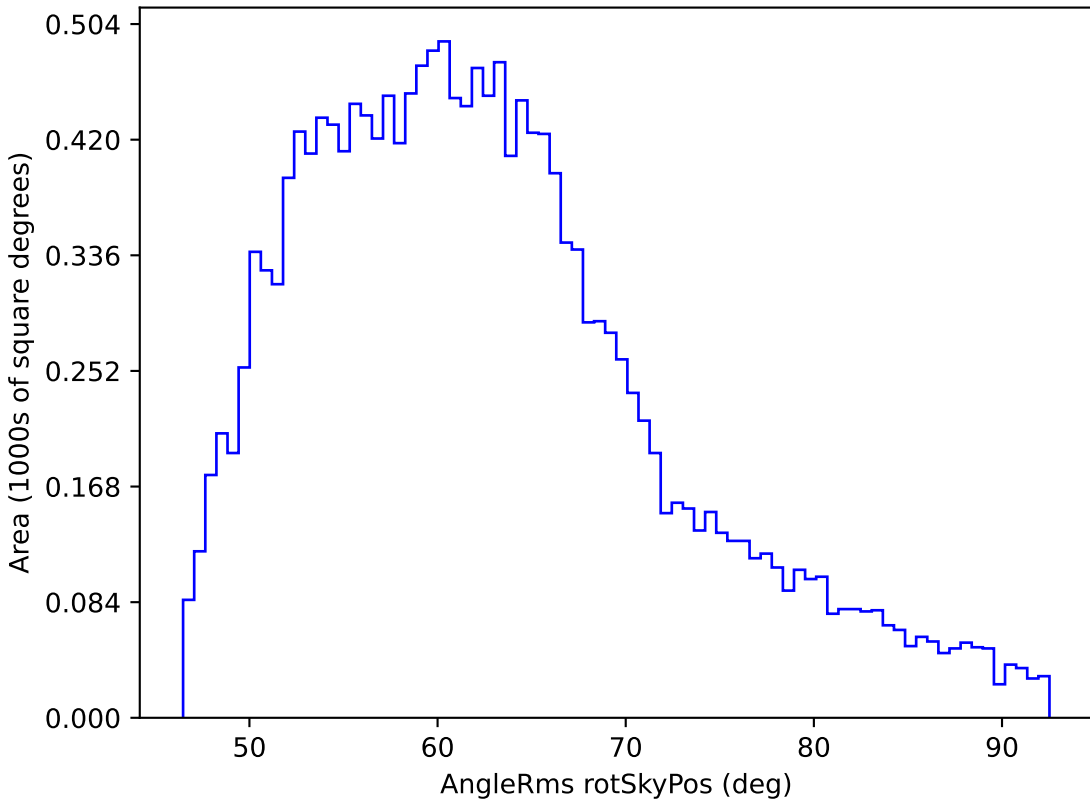
too_5_1v3.4_10yrs WFD y band: AngleRms rotSkyPos
