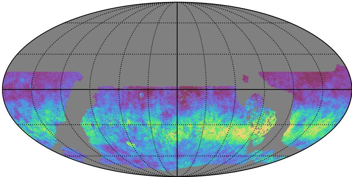
too_5_1v3.4_10yrs WFD u band: AngleRms rotSkyPos
