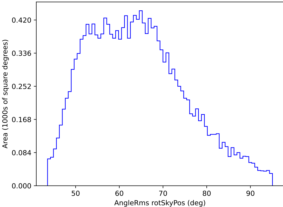
too_5_1v3.4_10yrs WFD u band: AngleRms rotSkyPos
