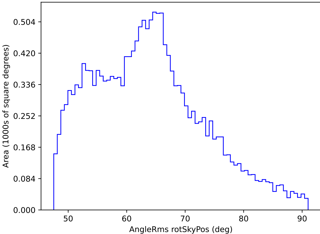
too_5_1v3.4_10yrs WFD i band: AngleRms rotSkyPos
