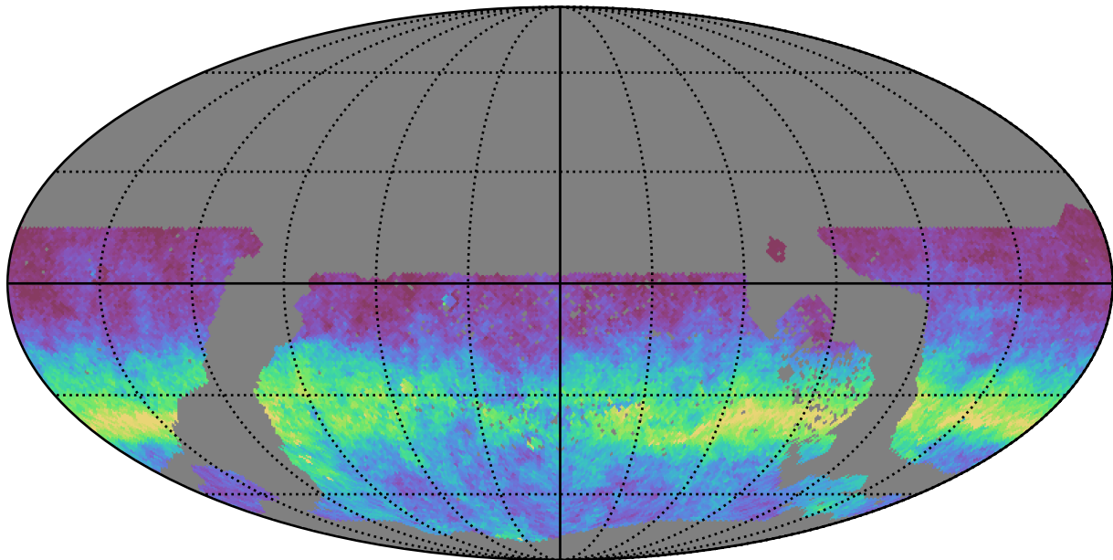
too_5_1v3.4_10yrs WFD g band: AngleRms rotSkyPos
