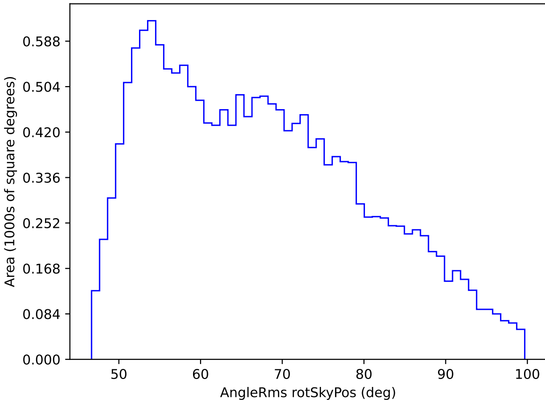
too_5_1v3.4_10yrs WFD g band: AngleRms rotSkyPos
