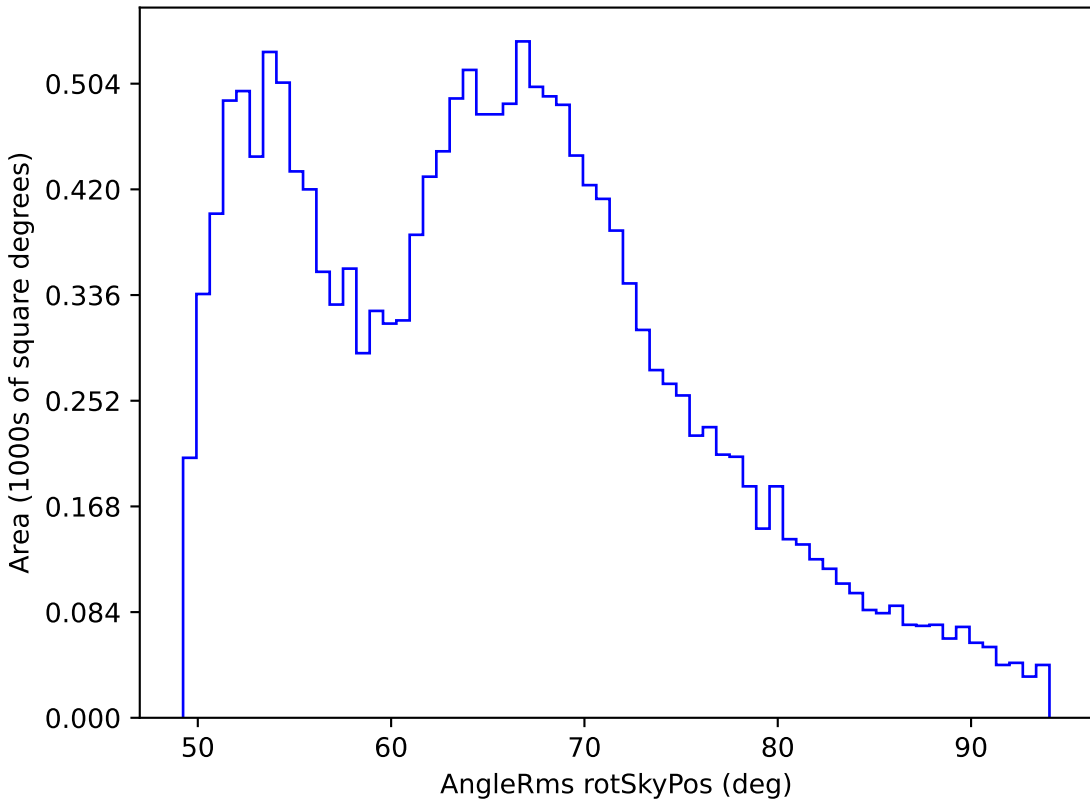
too_5_1v3.4_10yrs WFD all bands: AngleRms rotSkyPos
