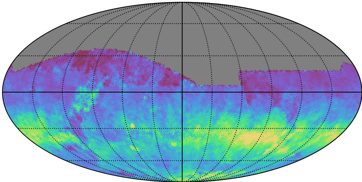
too_5_1v3.4_10yrs All sky z band: AngleRms rotSkyPos
