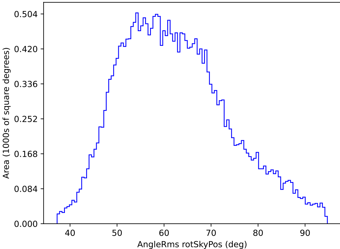
too_5_1v3.4_10yrs All sky z band: AngleRms rotSkyPos
