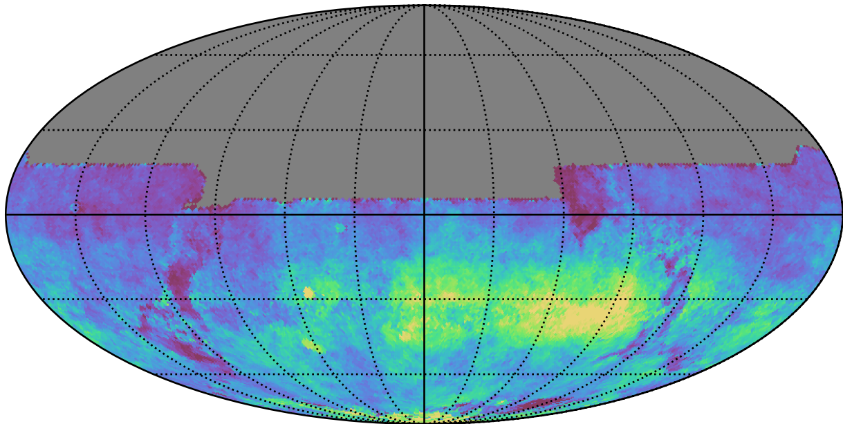
too_5_1v3.4_10yrs All sky y band: AngleRms rotSkyPos
