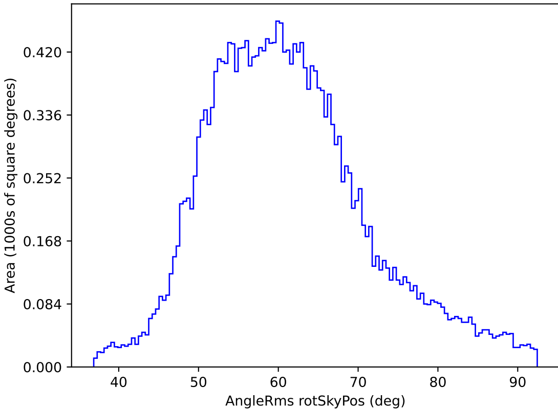
too_5_1v3.4_10yrs All sky y band: AngleRms rotSkyPos
