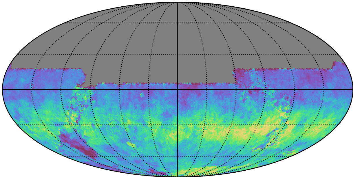
too_5_1v3.4_10yrs All sky u band: AngleRms rotSkyPos
