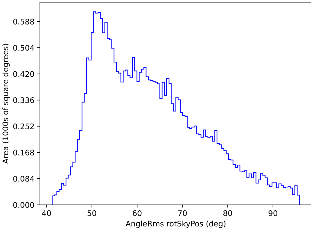
too_5_1v3.4_10yrs All sky r band: AngleRms rotSkyPos
