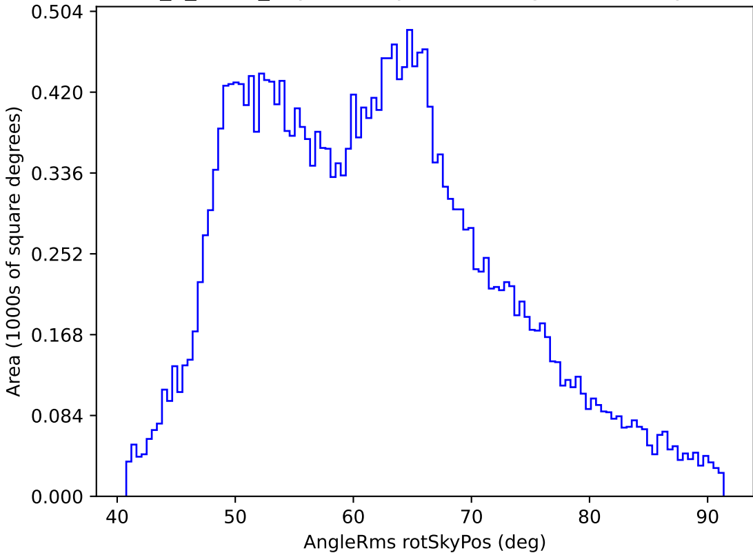
too_5_1v3.4_10yrs All sky i band: AngleRms rotSkyPos
