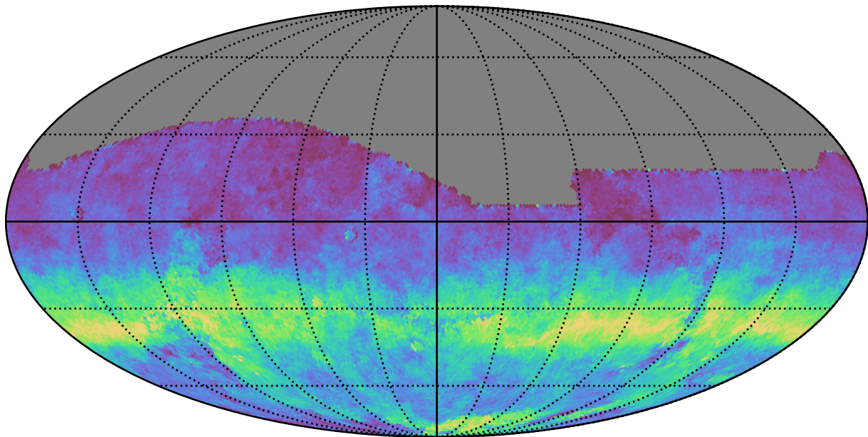
too_5_1v3.4_10yrs All sky g band: AngleRms rotSkyPos
