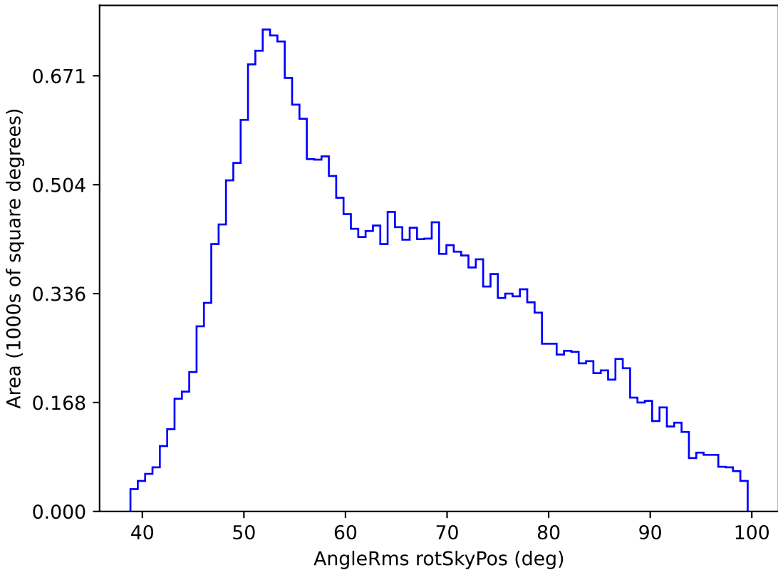
too_5_1v3.4_10yrs All sky g band: AngleRms rotSkyPos
