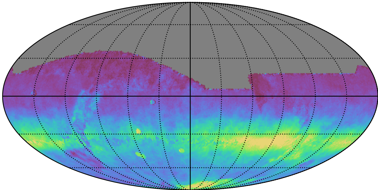
too_5_1v3.4_10yrs All sky all bands: AngleRms rotSkyPos
