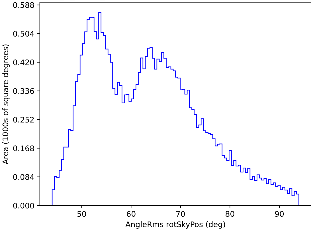
too_5_1v3.4_10yrs All sky all bands: AngleRms rotSkyPos
